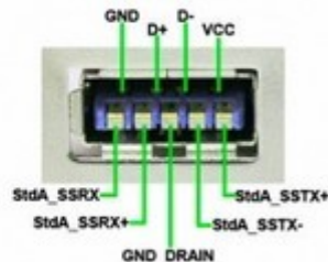
SuperSpeed standard A plug pinout
