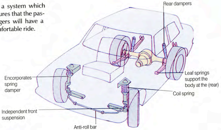
Suspension systems
