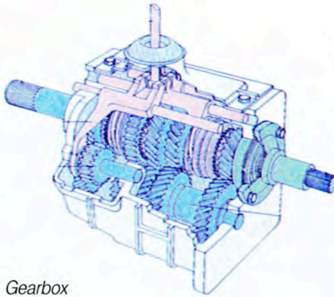
Gearbox
