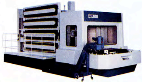
Tool-storage magazine
