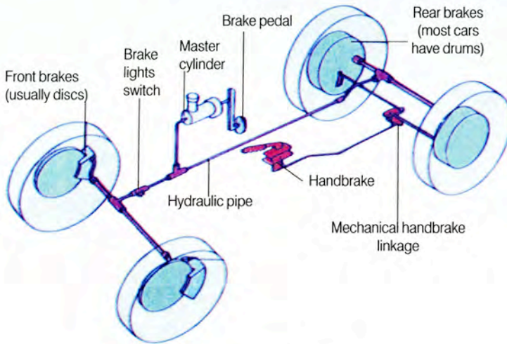
Braking system
