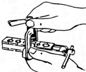
26. Flaring tubes
