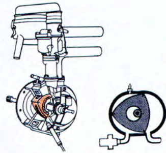
INTERNAL COMBUSTION ROTARY ENGINE (WANKEL)
