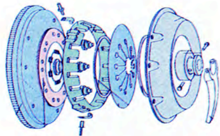
The parts of a diaphragm clutch
