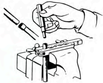
27. Swaging tubes
