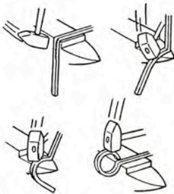
10. Forging
