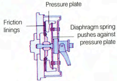
Clutch engaged
