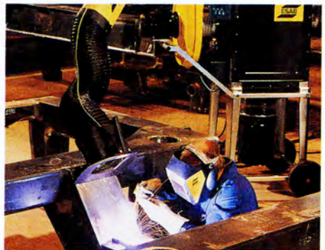
Proper dressing for the job to be done (overall, fire-proof gloves, face shield and shop cup)
