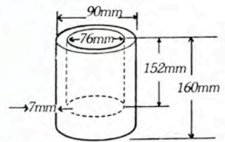
10. Cylindrical metal container
