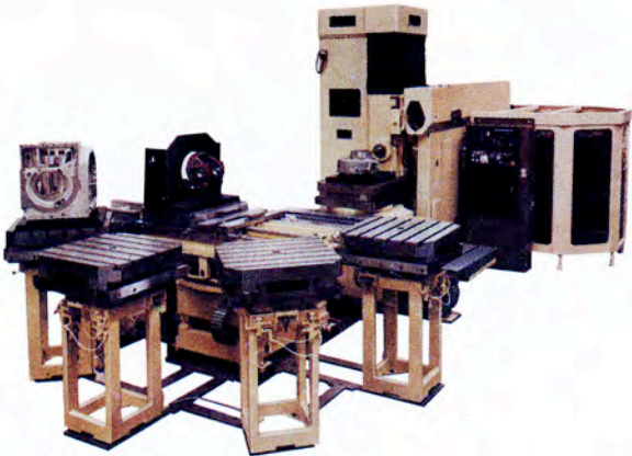
Pallet changing system
