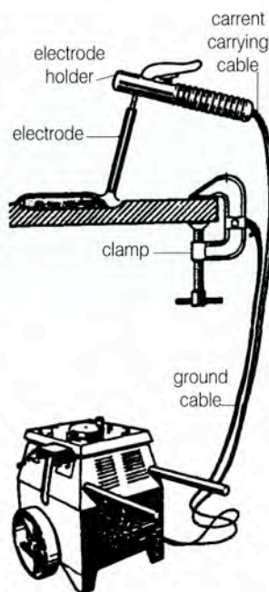
Welding machine
