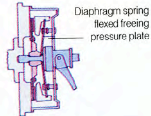
Clutch disengaged
