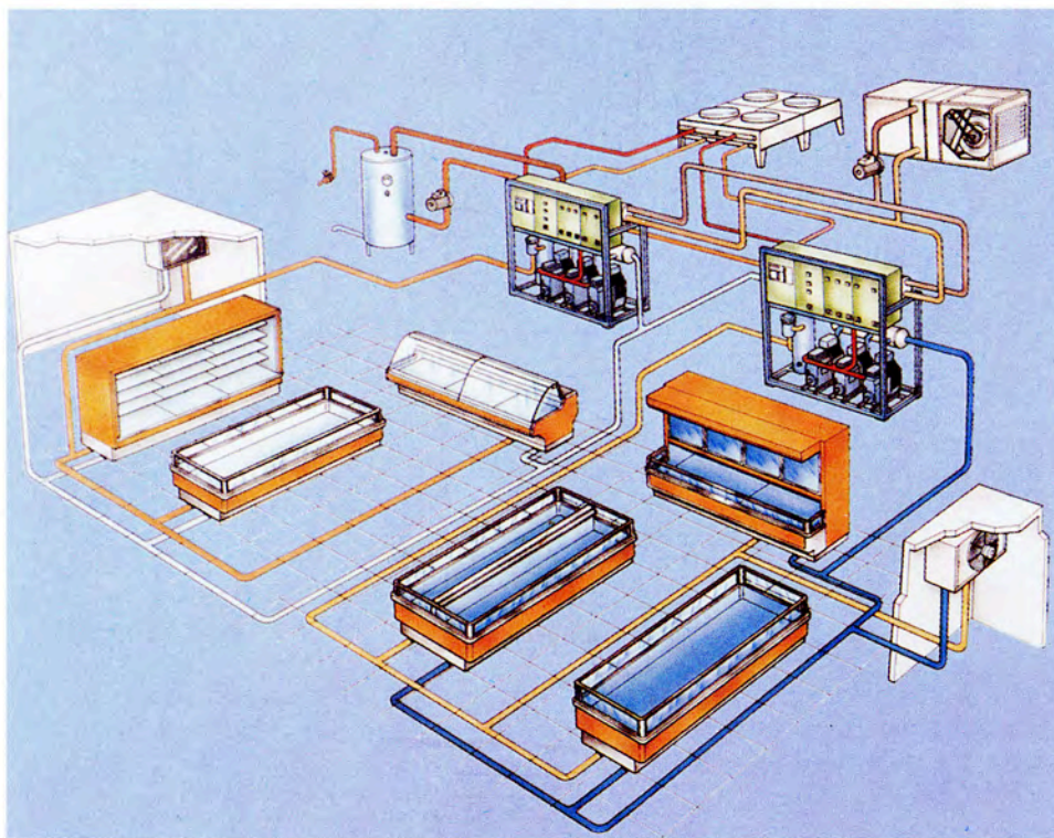
Commercial multi-compressor refrigeration system installed in a super-market
