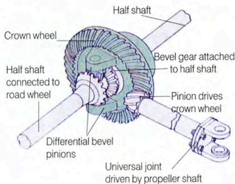
Differential
