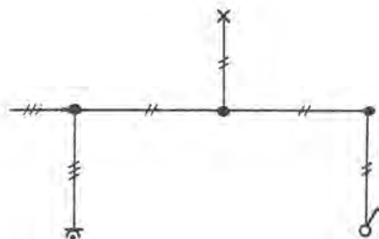
Single-pole representation
