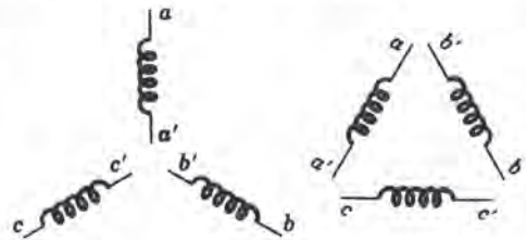
Star (Y) connection
