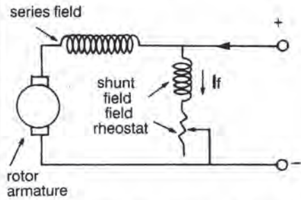
a) Compound excitation DC motor
