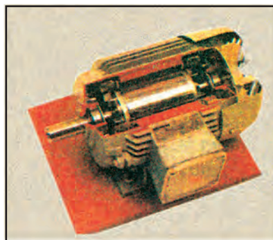
Three-phase induction motor with squirrel-cage rotor
