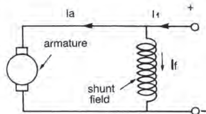
c) Shunt excitation DC motor
