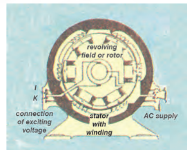
Single-phase AC generator
