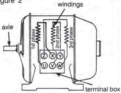
Windings of a three-phase asynchronous AC motor
