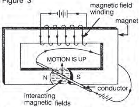
Producing mechanical force by passing current through a conductor lying in a magnetic field
