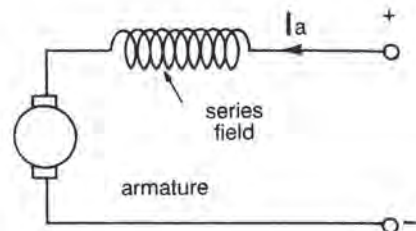
d) Series excitation DC motor
