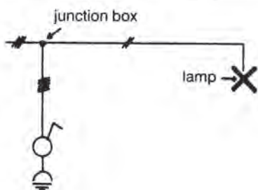
Figure 1. Wiring diagram presenting the exact location of the wiring and components of the circuit in the workshop
