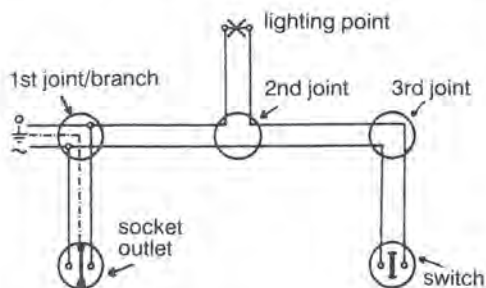
Multi-pole representation
