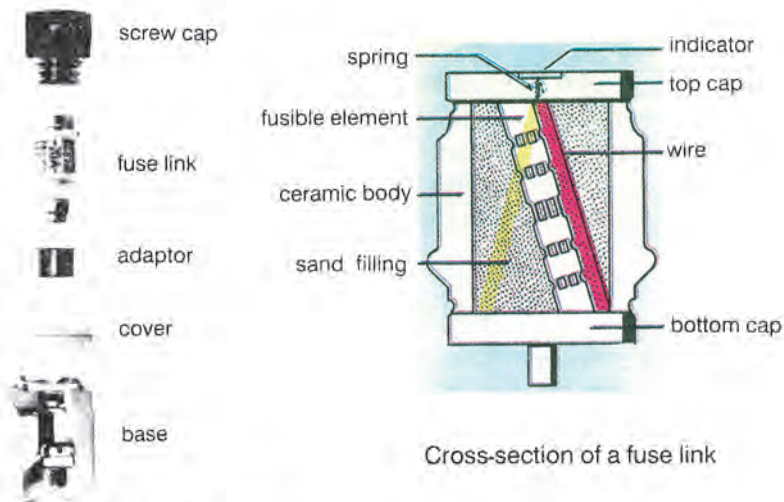
Parts of a fuse link
