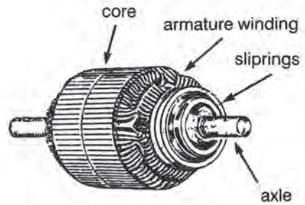
Rotor of an AC generator
